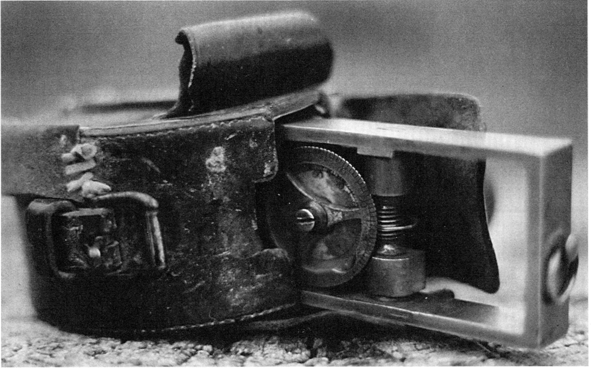
Fig. 7. Odometer from the 1850s. Odometers were commonly used by surveyors and the military during the Utah pioneer period. This odometer was probably employed by John W. Gunnison during his last survey. Shortly after he was massacred by natives in 1853 south of Delta, Utah, the pioneers recovered all of his equipment except his odometer. Some years later, this odometer was found on a trail near the massacre site.
